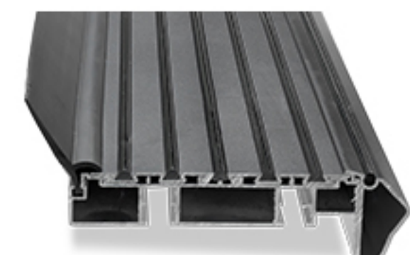
Three-layer thickening
